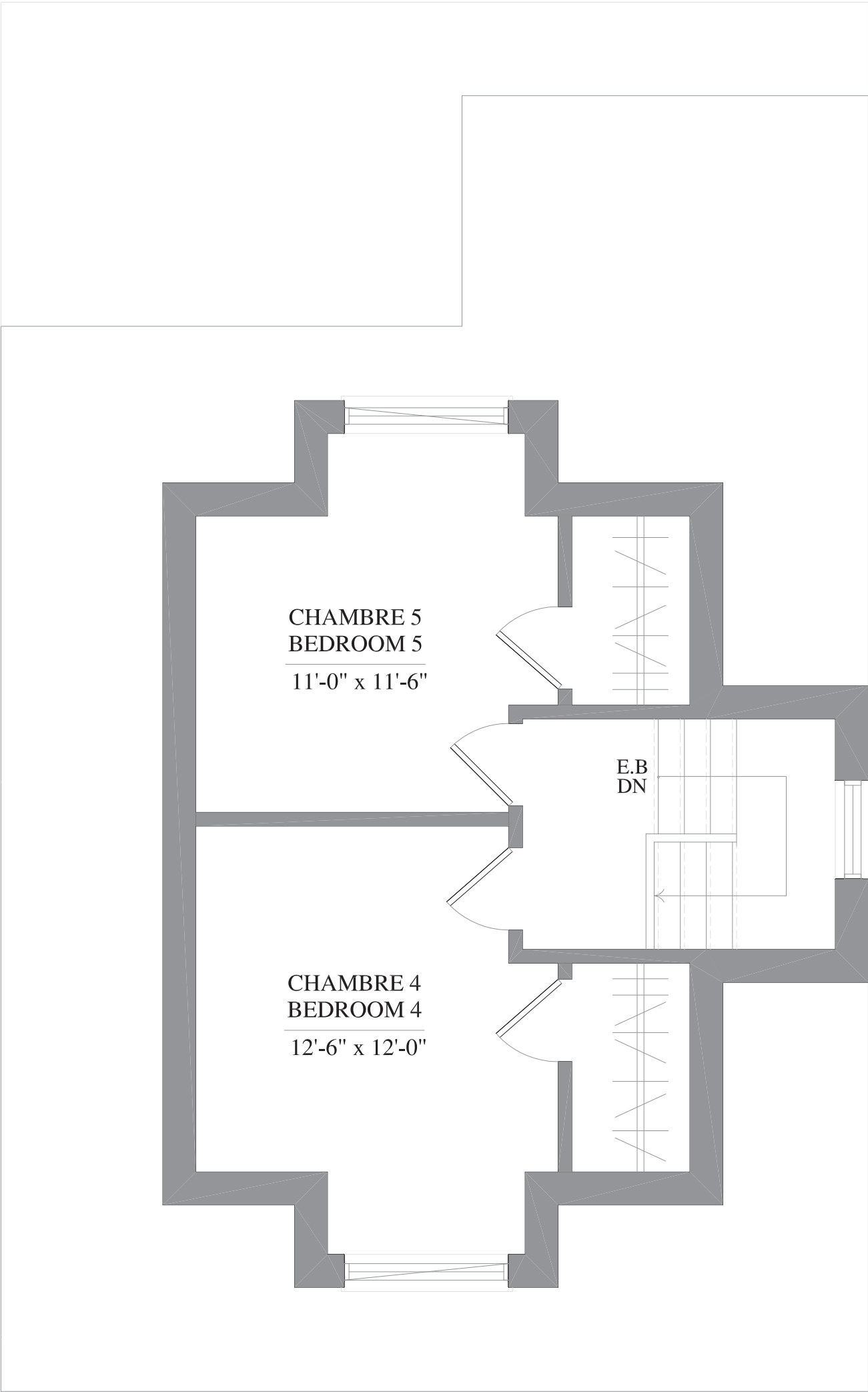
PLAN DU 3 ieme ETAGE THIRD FLOOR PLAN
